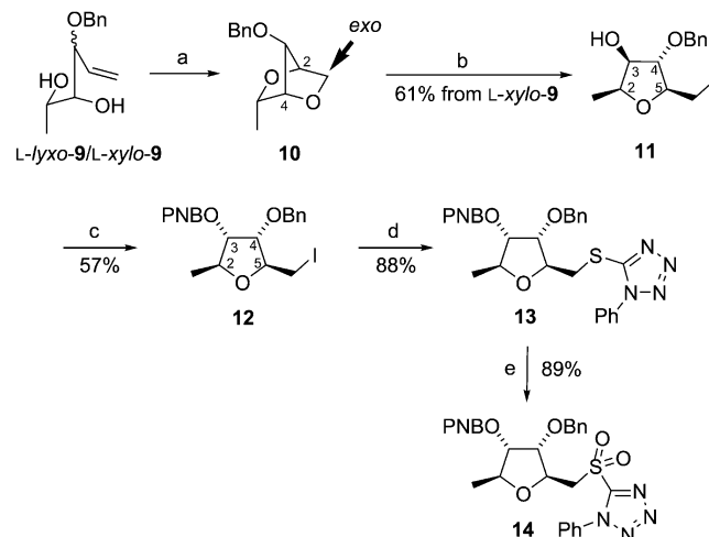
Scheme 3. Synthesis of sulfone 14 . Reagents and conditions: (a) PdCl 2 (0.1 equiv.), CuCl 2 (3 equiv.), AcONa (3 equiv.), AcOH, room temp., 12 h; (b) TMSCl, TBAI, HCl, CH 2 Cl 2 , room temp., 2 d, 61% from L-xylo-9; (c) DIAD (5 equiv.), Ph 3 P (5 equiv.), p -NBA (5 equiv.), reflux, 2 h, 57%; (d) KSPT, DMF, room temp., 8 h, 76%; (e) Mo VI /H 2 O 2 , EtOH, THF, 0 °C to room temp., 10 h, 89%. TMSCl = trimethylsilyl chloride, TBAI = tetrabutylammonium iodide, DIAD = diisopropyl azodicarboxylate, p -NBA = p -nitrobenzoic acid, KSPT = potassium 1-phenyl-1 H -tetrazol-5-thiolate, PNB = p -nitrobenzoyl.
