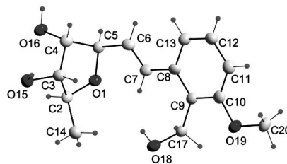
Figure 2. An ORTEP view of the crystal and molecular structure of natural (+)-varitriol [(+)- 1 ].
