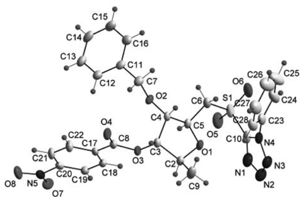
Figure 1. An ORTEP view of the crystal and molecular structure of sulfone 14 .
