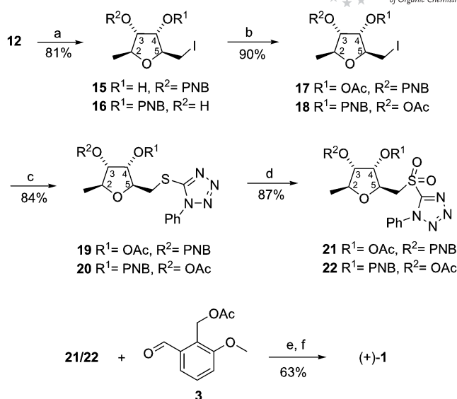
Scheme 4. Synthesis of varitriol ([+]-1). Reagents and conditions: (a) \text{BCl}_3 , \text{CH}_2\text{Cl}_2 , -50^\circ\text{C} , 50 min, 81% (71:29); (b) \text{Ac}_2\text{O} , DMAP, pyridine, room temp., 3 h, 90% (50:50); (c) KSPT, DMF, room temp., 8 h, 84% (50:50); (d) \text{Mo}^{\text{VI}}/\text{H}_2\text{O}_2 , EtOH, THF, 0^\circ\text{C} to room temp., 10 h, 87% (50:50); (e) KHMDS (1.4 equiv.), DME, -55^\circ\text{C} to room temp., 10 h; (f) NaOMe, MeOH, room temp., 4 h, 63% over 2 steps. DMAP = 4-(dimethylamino)pyridine, KHMDS = potassium hexamethyldisilazane.
