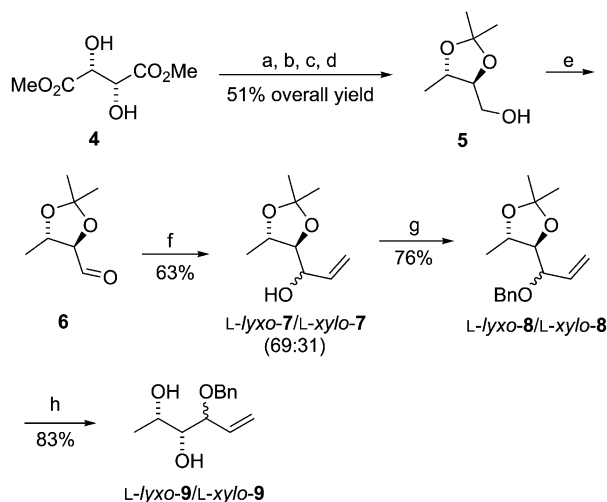
Scheme 2. Synthesis of L-xylo-9/L-lyxo-9. Reagents and conditions: (a) ref. [15] DMP, PTSA, benzene, 98%; (b) ref. [16] NaBH 4 , MeOH, 80%; (c) ref. [17] TsCl, Bu 4 NHSO 4 , 15% NaOH, CH 2 Cl 2 , 86%; (d) ref. [17] LAH, Et 2 O, 76%; (e) (COCl) 2 , DMSO, Et 3 N, CH 2 Cl 2 , -78 °C to room temp., 2 h; (f) vinylmagnesium bromide, THF, 0 °C to room temp., 12 h, 63% from 5 ( anti / syn , 69:31); (g) BnBr, NaH, DMF, 0 °C to room temp., 12 h, 76%; (h) 60% AcOH, room temp., 10 h, 83%. DMP = 2,2-dimethoxypropane, PTSA = p -toluenesulfonic acid.
